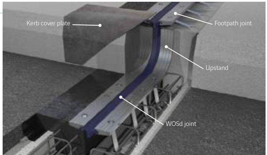
3D view of the upstand
