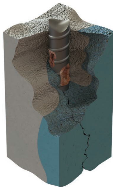
Corrosion damage
