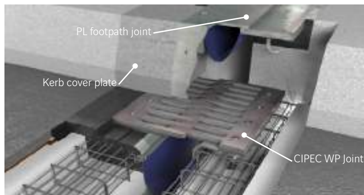
3D view of the footpath
