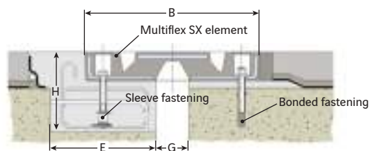
Single element module
