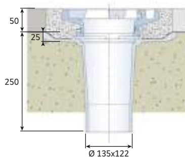
Basic assembly with one riser
