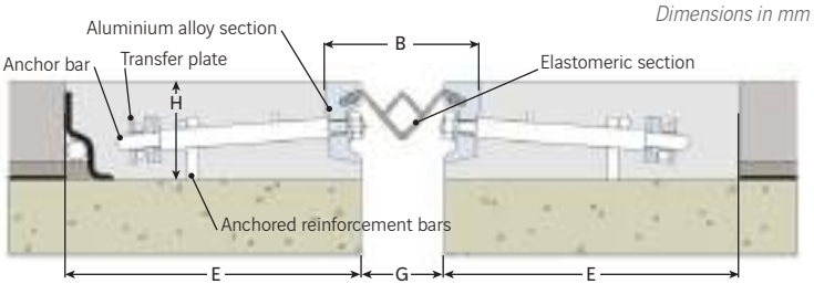
WRB with anchor bars
