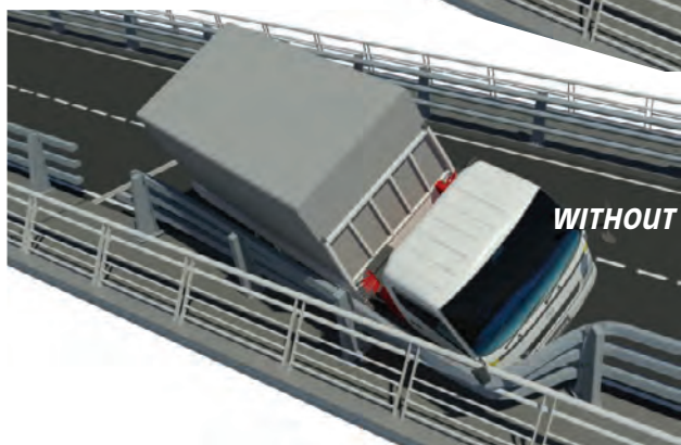
Simulation of a collision on a crash barrier with or without the Transpec 4-18
