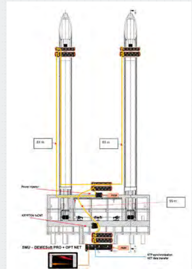
Figure 5. Overall measurement instrumentation setup on pylons and bridge structure.
