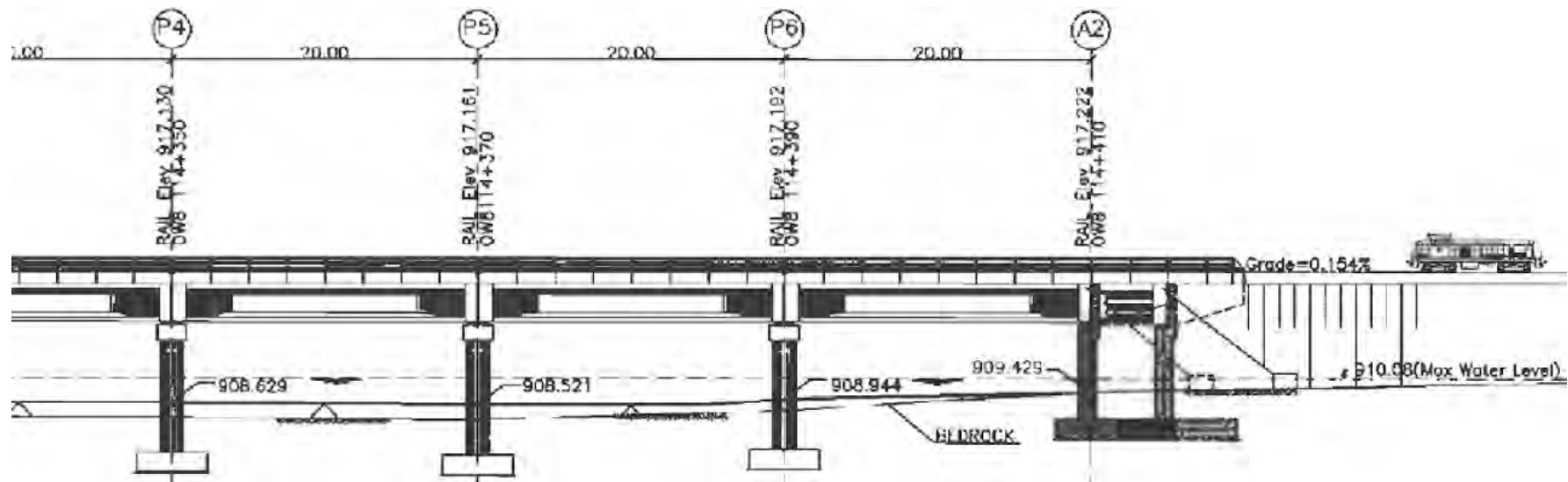
Figure 2. Bridge design – the High Mileage Elevation.
