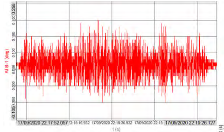
Figure 10. Software recordings from a tilt-meter monitoring tilt/inclination response for the sensor "B" located at the girder MGI2 soffit when a phosphate train passed the bridge on September 17th, 2020.
