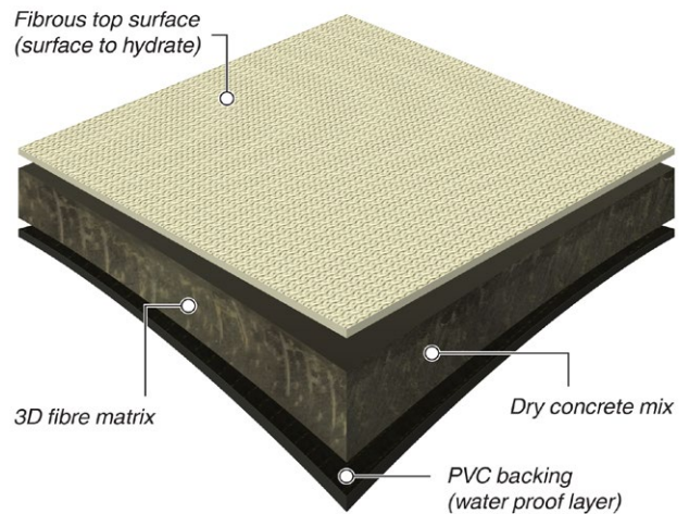
Concrete Canvas® GCCM Section
